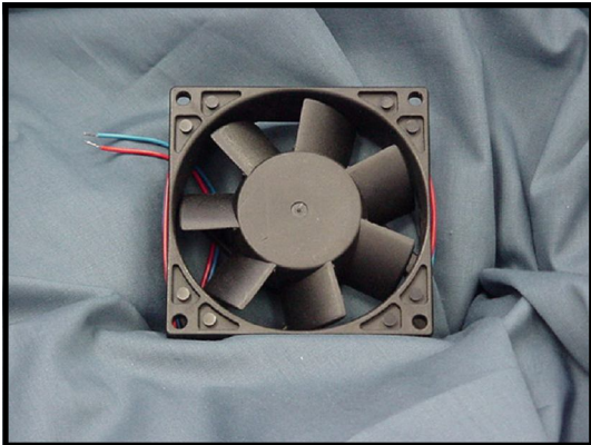
SIZE: 80 x 80 x 25.4 mm [3.1 x 3.1 x 1.0 inches] WEIGHT: 125 grams $10.25 each (1-50 units)
