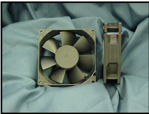
SIZE: 92 x 92 x 38 mm. [3.6 x 3.6 x 1.0 inches] WEIGHT: 170 grams $10.25 each (1-50 units)
